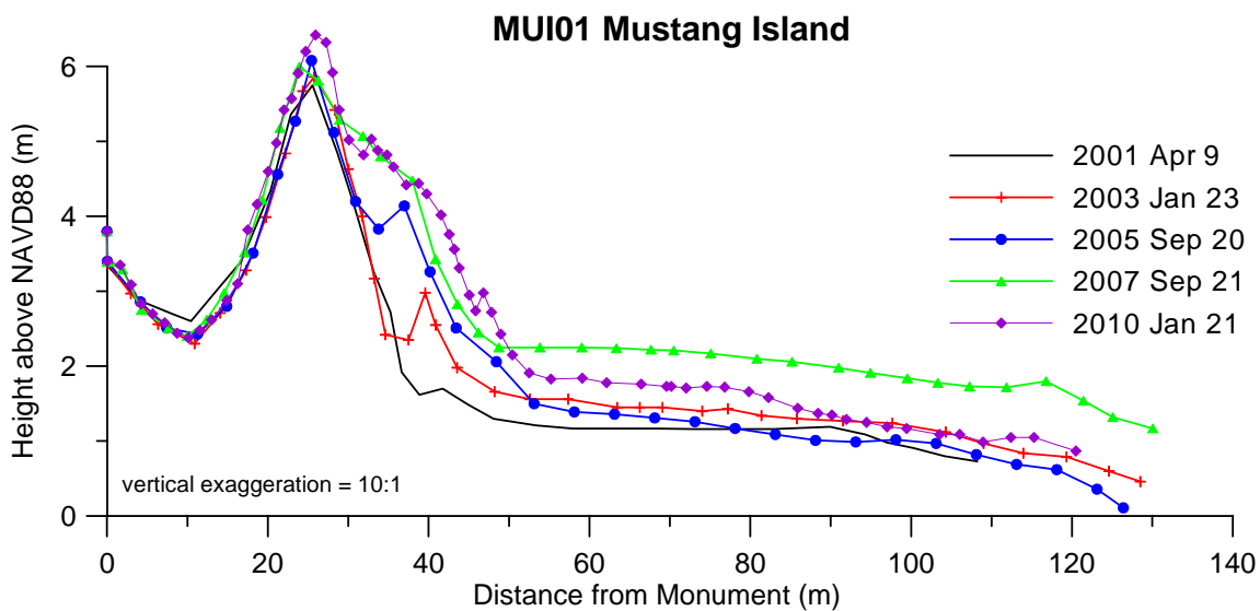
Figure 12. Foredune expansion at MUI01 on Mustang Island.
