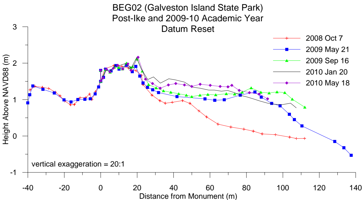
Figure 10. Beach profile plots from BEG02 in Galveston Island State Park. Top graph shows the post-Hurricane Ike profile compared with two prestorm profiles from early 2008 and the post-Tropical Storm Frances profile from September 1998. The old datum marker is 0. The bottom graph (BEG02 reset datum) shows poststorm profiles plus data collected by Ball High School students during the 2009–2010 academic year. Students are monitoring recovery of the beaches and dunes at this site.
