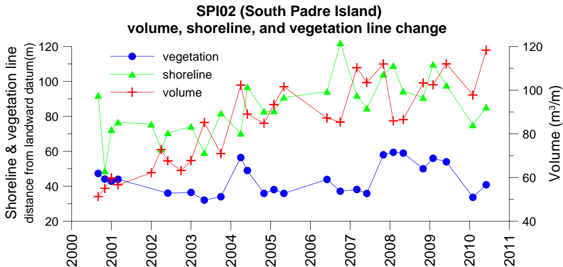
Figure 11. Changes at SPI02 on South Padre Island due to installation of sand fence and beach nourishment.
