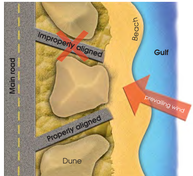
Figure 26. Alignment of beach access roads.
