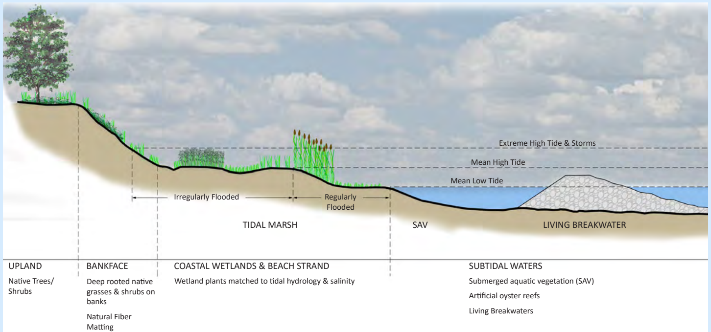
Coastal Shoreline Continuum and Typical Living Shorelines Treatments. 1 Photo: Allen Engineering and Science
