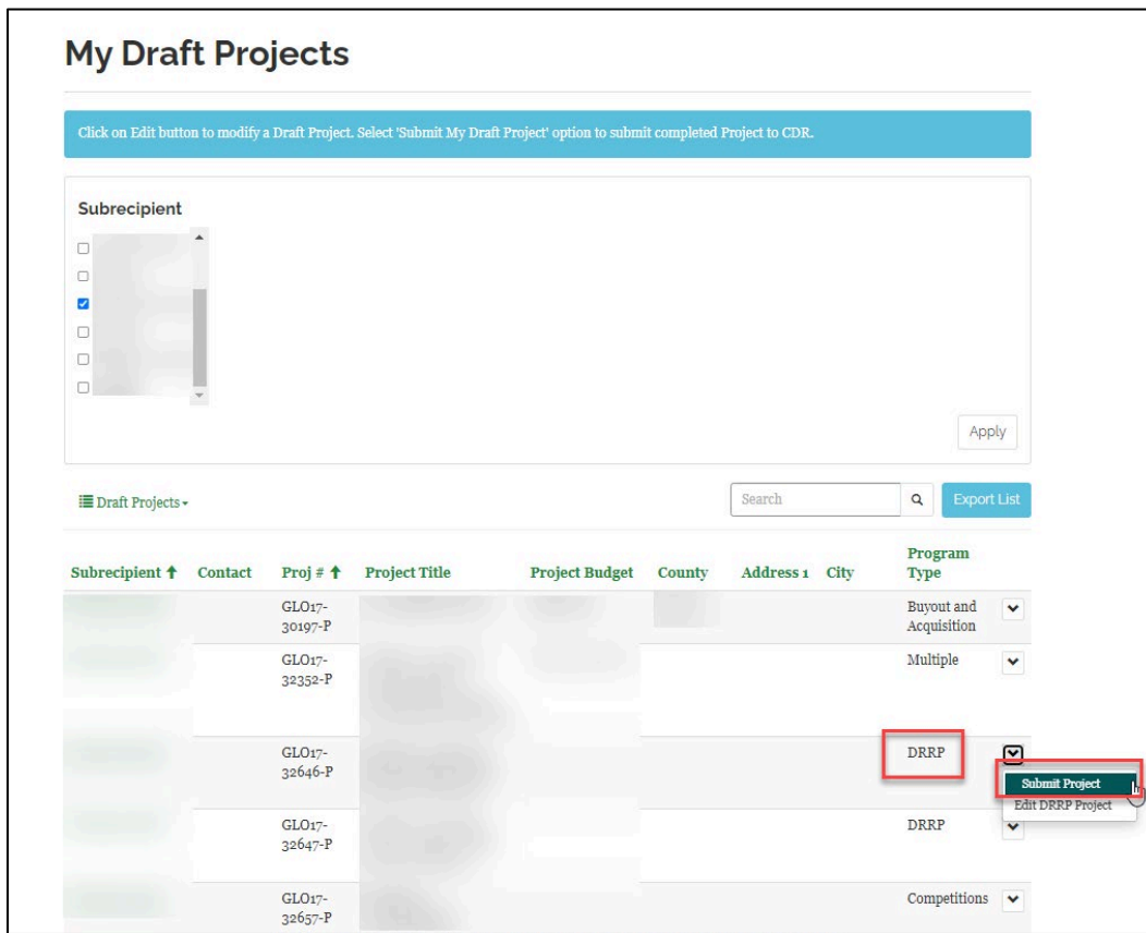
Figure 58: Application Submission-Project
