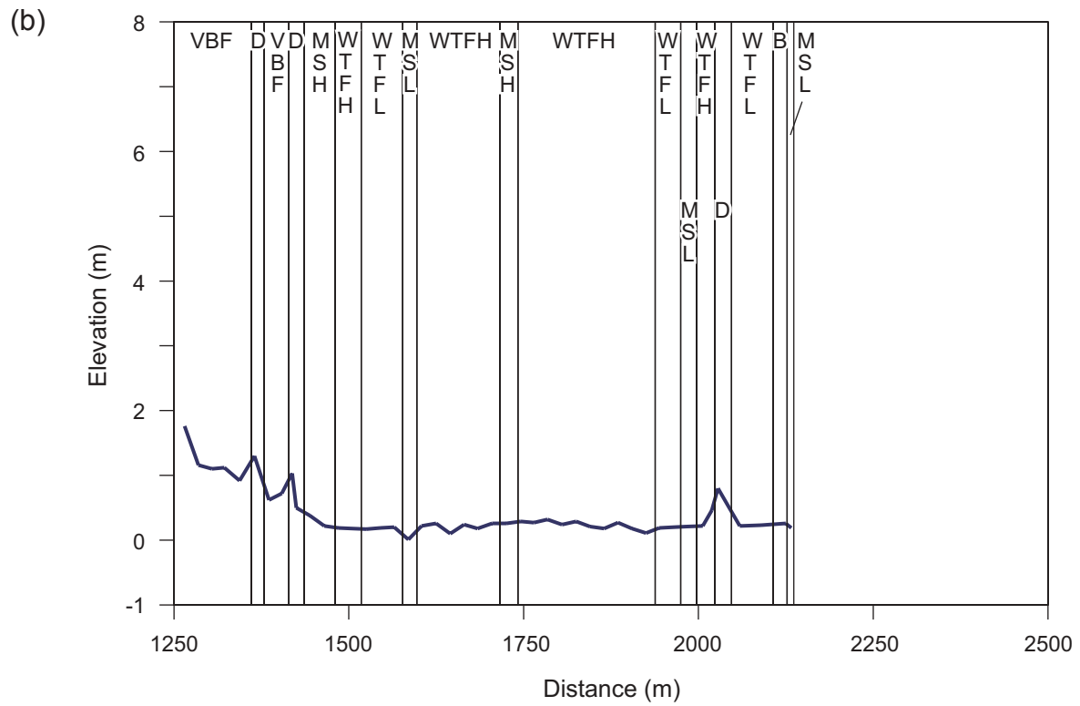
Figure 21. Elevation profile superimposed with surveyed coastal environments along the MISIP transect (a) between 0 and 1250 m and (b) between 1250 and 2200 m from the gulf shoreline.
