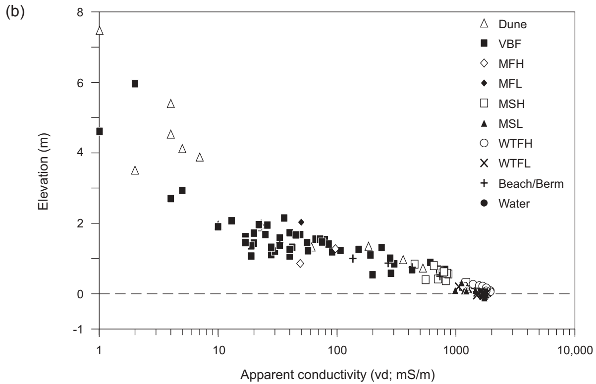
Figure 37. Elevation and apparent conductivity of (a) 1992 NWI units, and (b) coastal environments along the PA transect. Apparent conductivity measured in the vd orientation.
