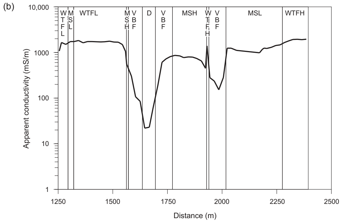
Figure 35. Apparent conductivity profile (vertical dipole orientation) superimposed with surveyed coastal environments along the PA transect (a) between 0 and 1250 m and (b) between 1250 and 2400 m from the gulf shoreline.
