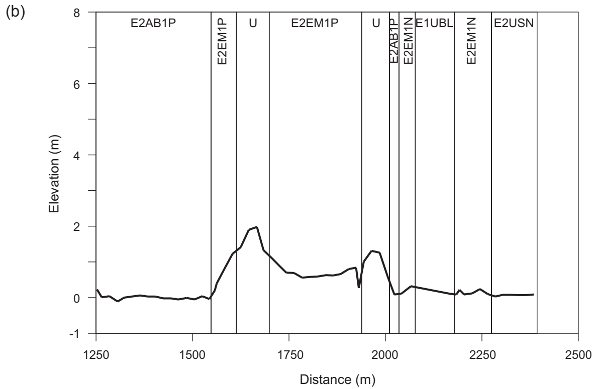
Figure 31. Elevation profile superimposed with 1992 NWI units along the PA transect (a) between 0 and 1250 m and (b) between 1250 and 2400 m from the gulf shoreline.
