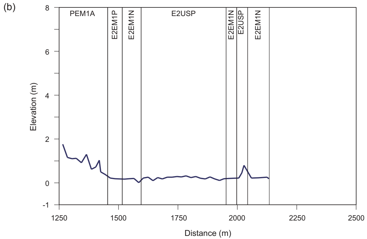
Figure 20. Elevation profile superimposed with 1992 NWI units along the MISIP transect (a) between 0 and 1250 m and (b) between 1250 and 2200 m from the Gulf shoreline.
