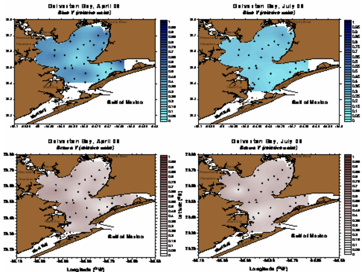
Fig. 14 Spatial maps of revealing the efficiency of photosynthesis (measured as Y or yield) for Cyanophyta (blue) and Dinophyta plus Bacillariophyta (brown) as measured with a PHYTO-PAM.
