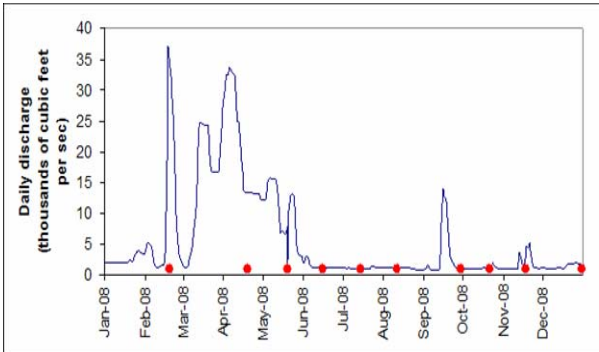
Fig. 4 Daily discharge of freshwater into Galveston Bay from January 01 to December 31 2008. Real-time flow data was downloaded from the USGS monitoring station located in the Trinity River at Romayor (08066500) located near the river’s mouth. Red spots indicate timing of monthly field trips.
