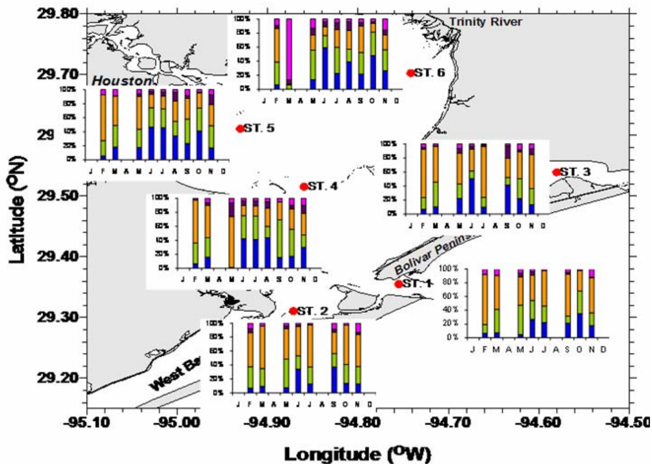
Fig. 12 Monthly changes in phytoplankton community composition throughout Galveston Bay during 2008 as measured at 6 fixed stations.
