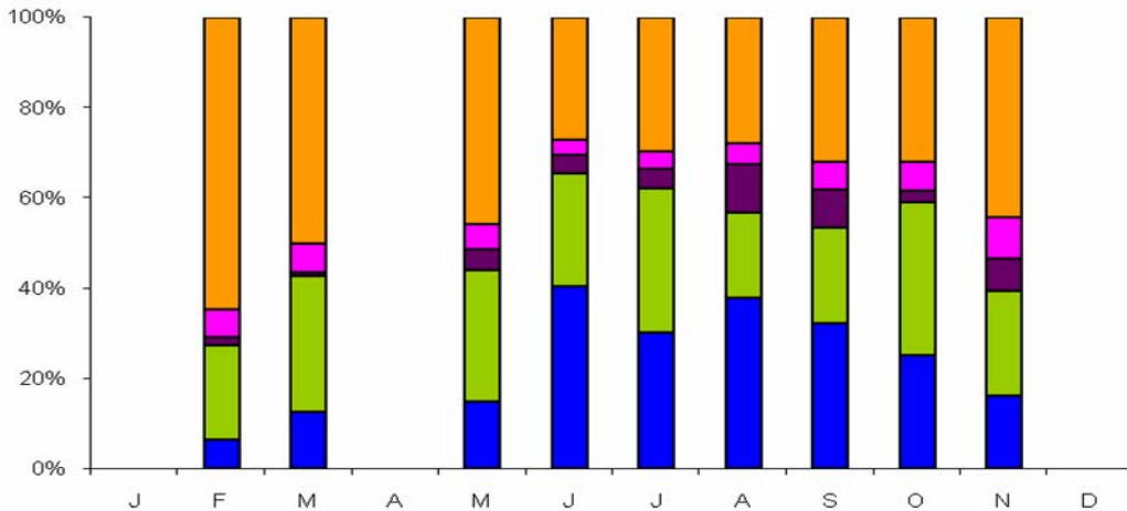
Fig. 13 Monthly changes in phytoplankton community composition in Galveston Bay during 2008 at all fixed stations.
