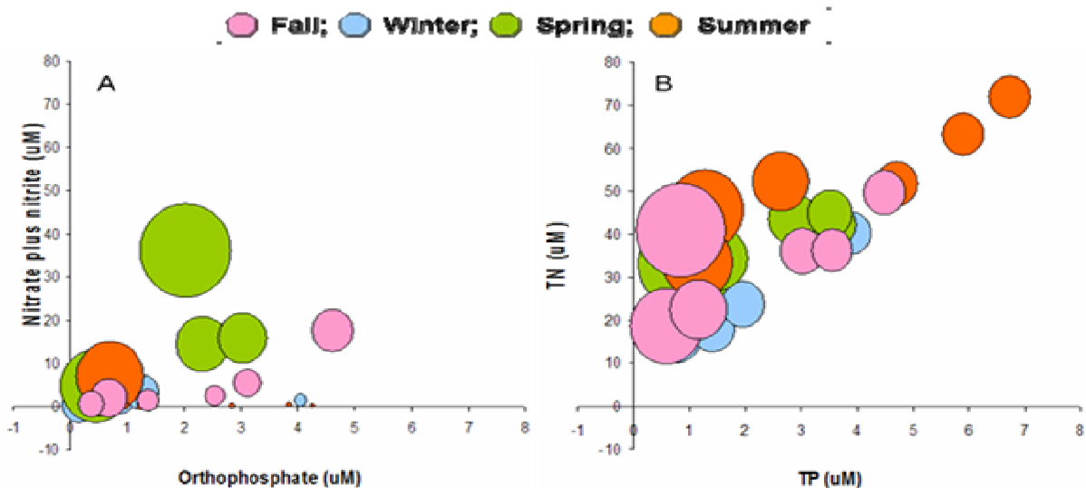
Fig. 9 Seasonal changes in dissolved (A, left) and total (B, right) nutrient concentrations (uM) in Galveston Bay. 9A: N as nitrate plus nitrite versus orthophosphate. 9B: TN versus TP. The x- and y-axis are concentrations; the bubbles were calculated as nutrient ratios and provide a visual of the magnitude of nutrients in each season.
