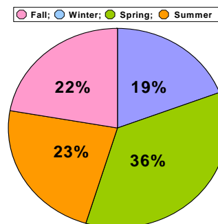
Fig. 11 Seasonal primary production (as a % of total).
