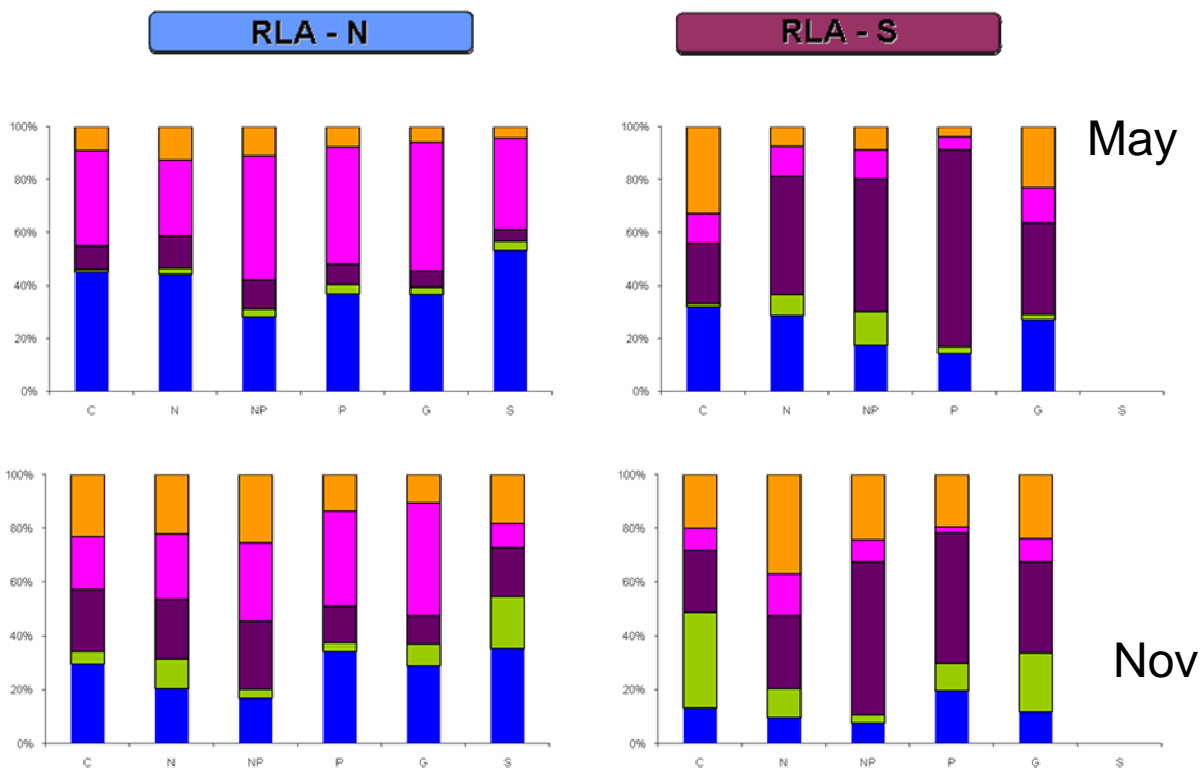
Fig. 16 Outcomes of the resource limitation assays. Assays were performed in the northern (left) and southern (right) sections of Galveston Bay during 2008. Changes in phytoplankton biomass were examined as changes in the distributions of the major phytoplankton taxa (color code key in section 4.6).
