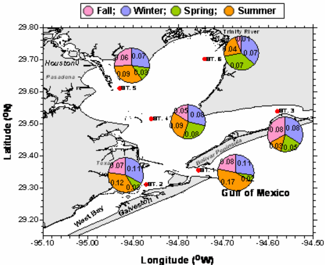
Fig. 6 Seasonal changes in total suspended sediment (TSS; mg/l) loads in Galveston Bay.
