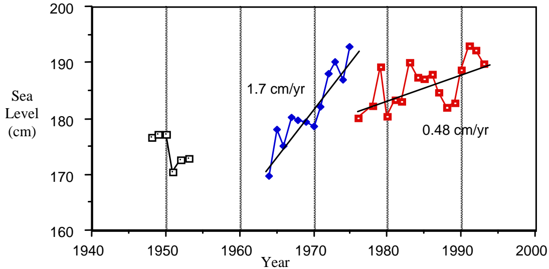
Figure 16. Sea-level rise at the Rockport tide gauge located near the landward margin of Aransas Bay. Tide data from NOAA.
