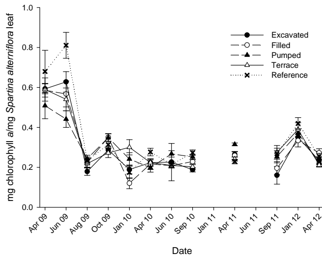
Figure 18: Chlorophyll a content of Spartina alterniflora leaves at various restoration sites and a reference area. Bars represent standard error. 6 \leq n \leq 10 . No data were collected in January or June 2011.
