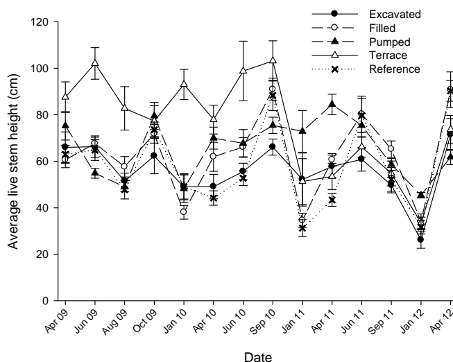
Figure 14: Average canopy height of all live species at various restoration sites and a reference area. Bars represent standard error. 6 \leq n \leq 10
