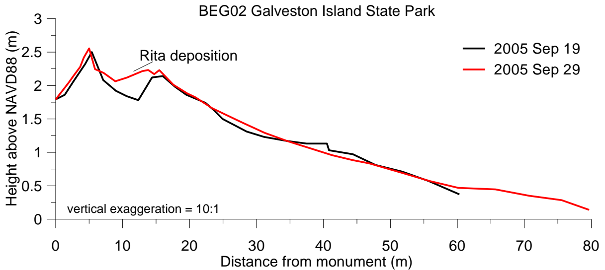
Figure 13. Plot of pre- and post-Rita beach profiles measured at Galveston Island State Park.
