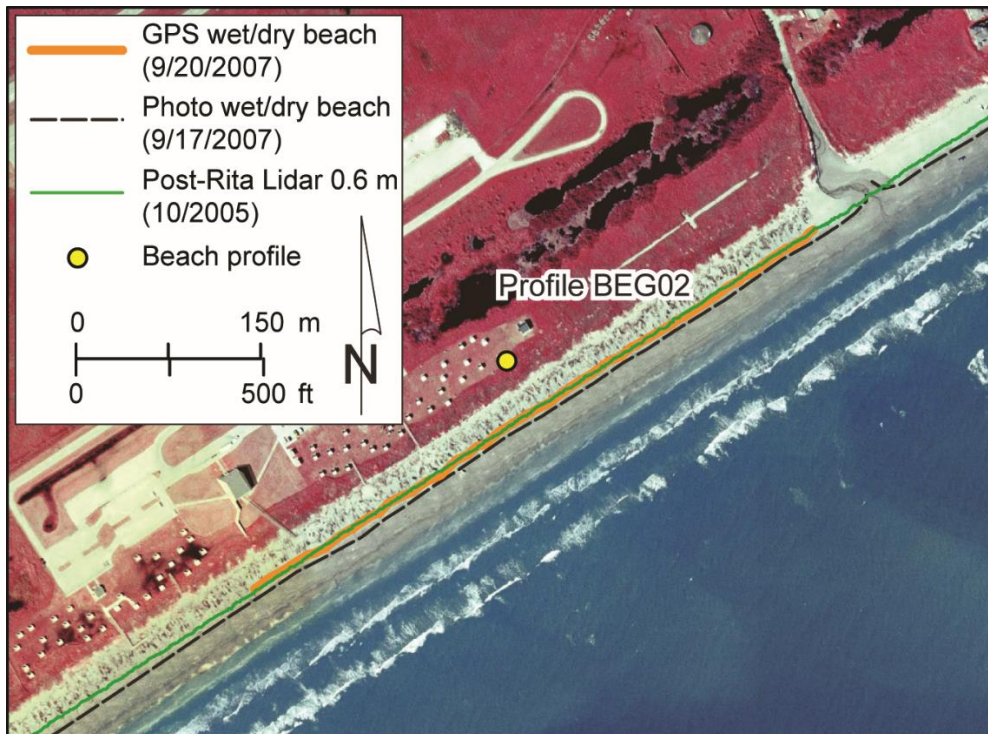
Figure 11. Shoreline position comparison at Galveston Island State Park site BEG02. Shorelines include the 2007 wet beach/dry beach boundary mapped on aerial photographs taken September 17, 2007; the wet beach/dry beach boundary mapped on September 20, 2007, by THSCMP students and staff using ground GPS; and the 0.6-m msl shoreline proxy extracted from airborne lidar data acquired after Hurricane Rita in October 2005. From Paine and others (2011).
