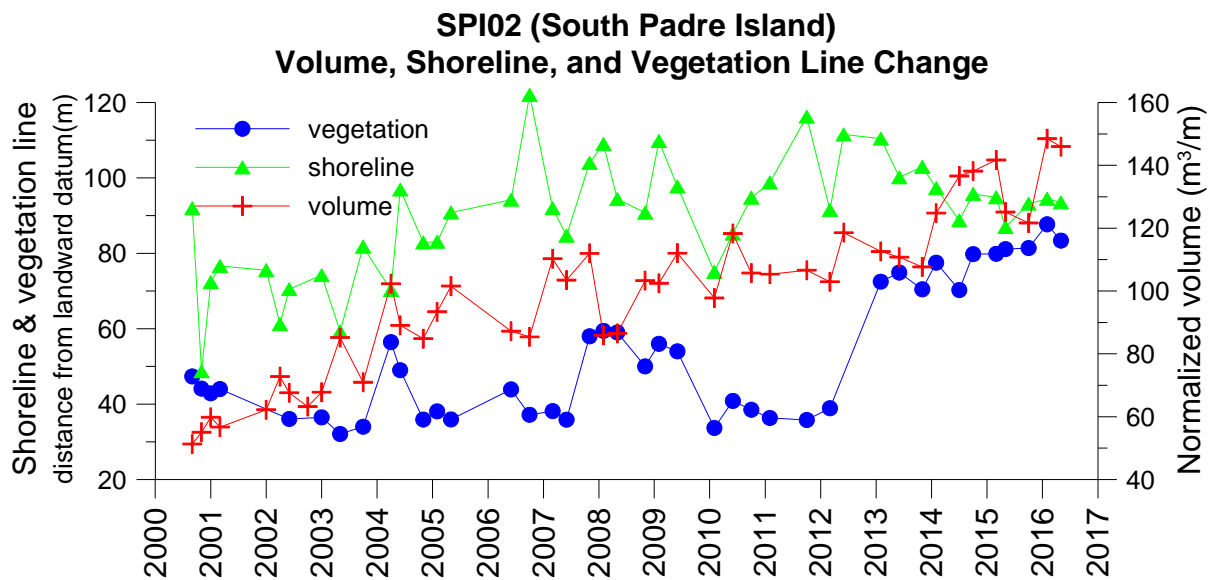
Figure 17. Changes at SPI02 on South Padre Island due to beach-nourishment projects and the installation of sand fences.
