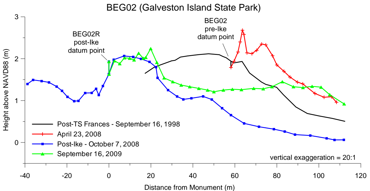
Figure 14. Beach-profile plots from BEG02 in Galveston Island State Park comparing the post–Hurricane Ike profile with a pre-storm profile from early 2008 and the post–Tropical Storm Frances profile from September 1998. Data from September 2009 (one year post-storm) is also included.
