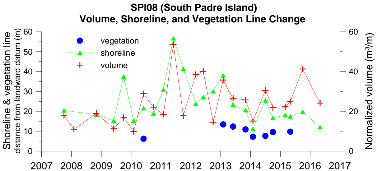
Figure 18. Volume and shoreline changes at SPI08 on South Padre Island due to beach-nourishment projects and the installation of sand fences.
