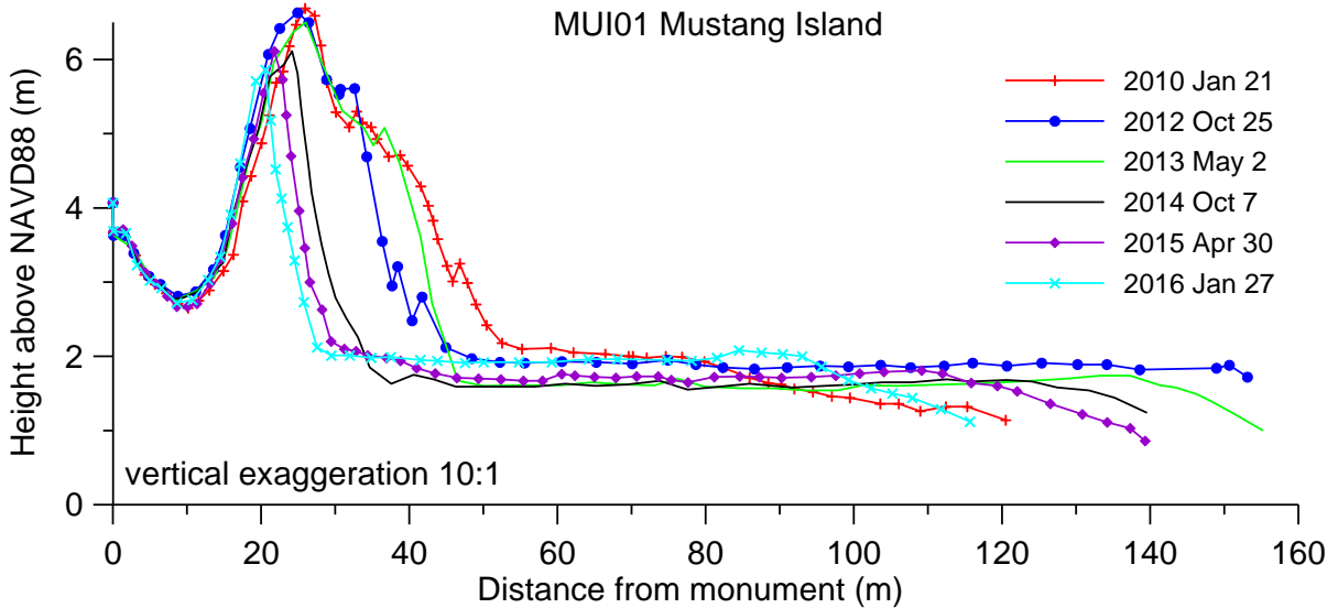
Figure 20. Excavated dune profile at MUI01 on Mustang Island.
