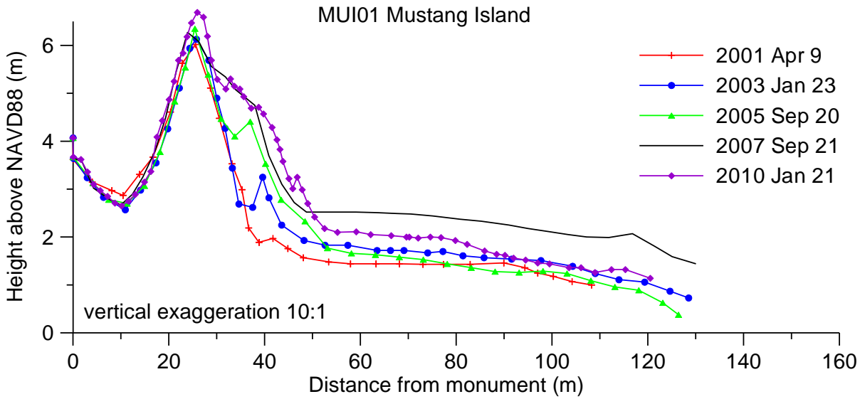
Figure 19. Foredune expansion at MUI01 on Mustang Island.
