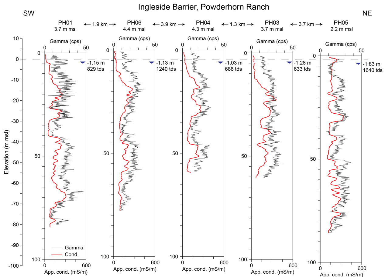
Figure 17. Well log cross section oriented southwest to northeast across Powderhorn Ranch showing gamma and conductivity logs from wells PH01, PH06, PH04, PH03, and PH05 (fig. 13). Also shown are measured water levels and total dissolved solids concentration estimated from water samples.
