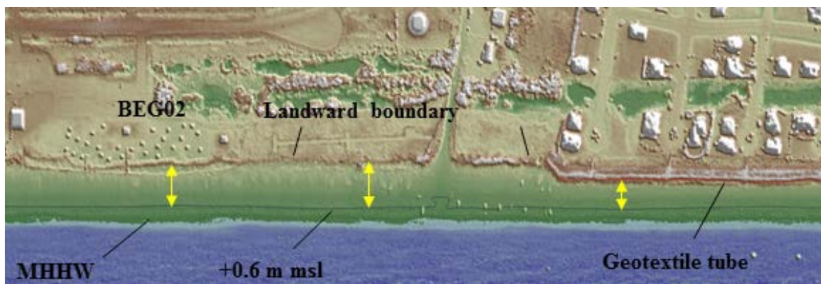
Figure 12. Lidar topographic-relief image of Galveston Island State Park and Pirates Beach subdivision. Note the difference in beach width between the natural beach and the area in front of the subdivision. From Gibeaut and others (2003).
