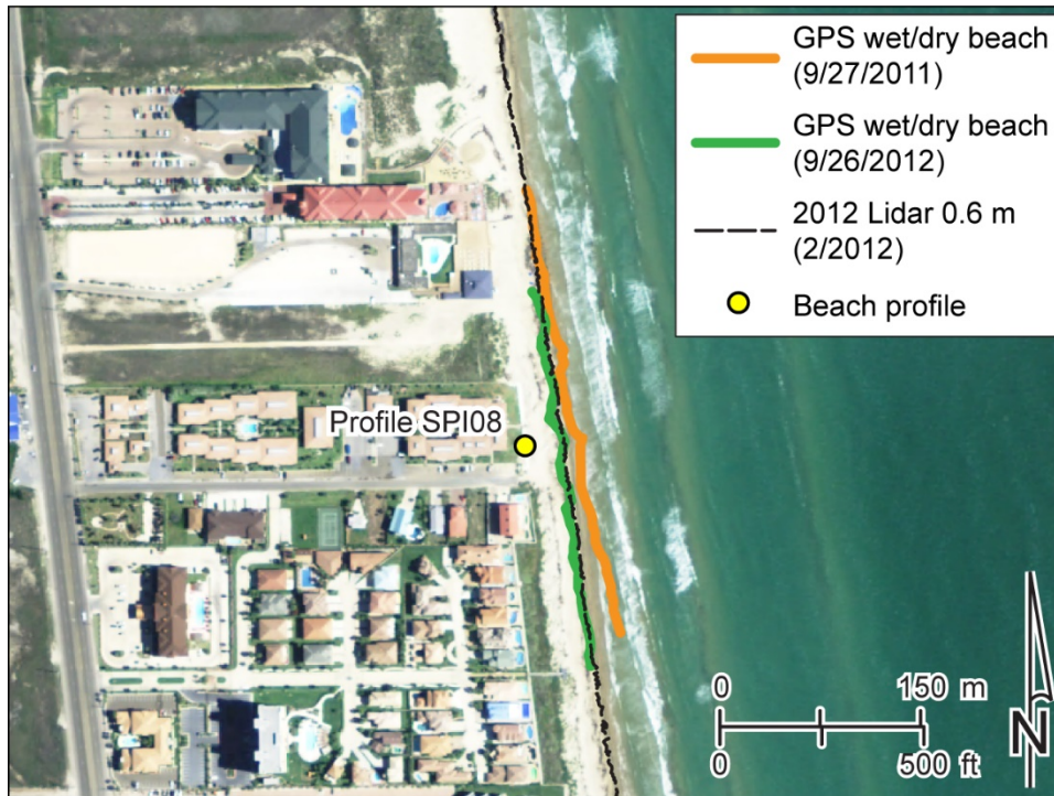
Figure 14. Shoreline position comparison at South Padre Island site SPI08. Shorelines include the wet beach/dry beach boundary mapped on September 27, 2011 and September 26, 2012 by THSCMP students using GPS and the shoreline proxy extracted from airborne lidar data acquired in February 2012. Shorelines are superimposed on NAIP imagery acquired on April 23, 2012. From Paine and others (2014).
