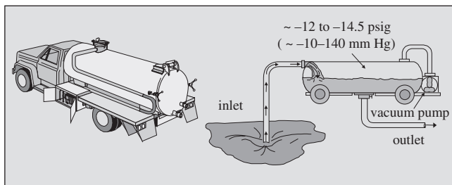
Figure 11-13 Vacuum Truck
