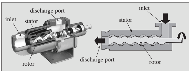
Figure 11-8 Progressive Cavity Pump
